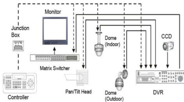
Controller Connectivity
